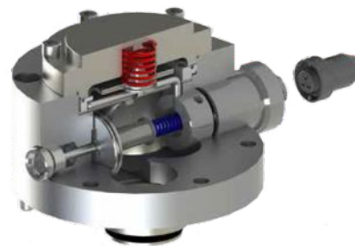
Bypass open
