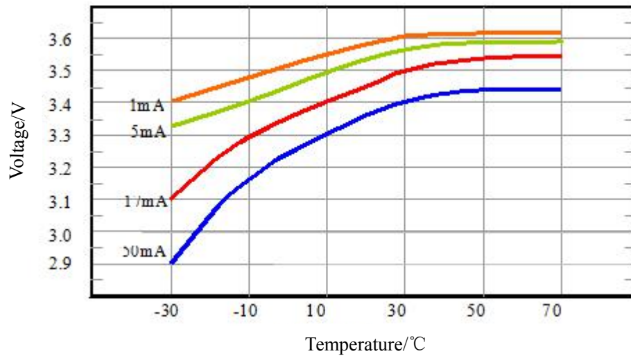
Voltage platform characteristic diagram at different temperatures
